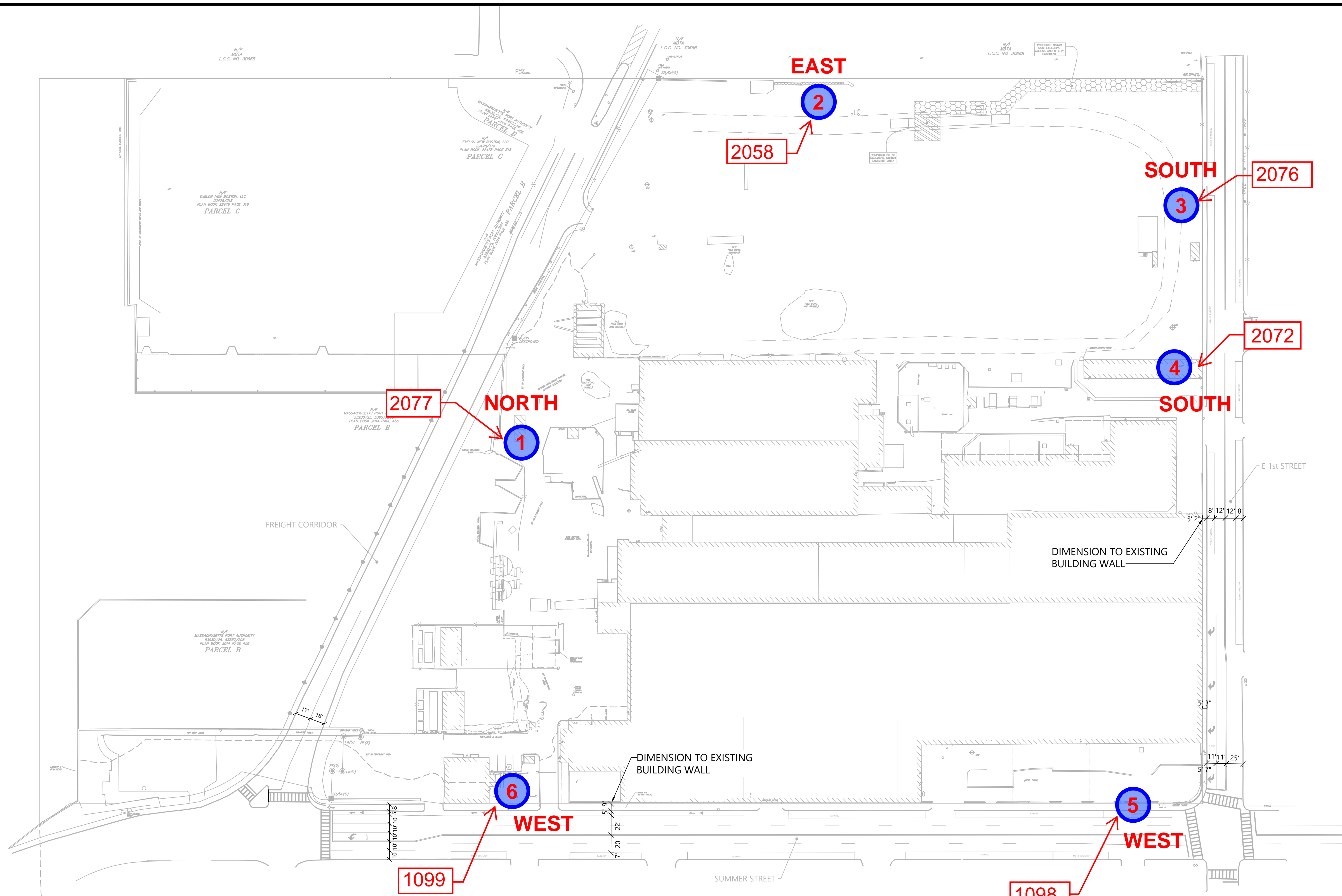
776 Summer Street - Deconstruction SOUTH BOSTON EXISTING CONDITIONS FIGURE 2 DUST MONITORING LOCATION PLAN
