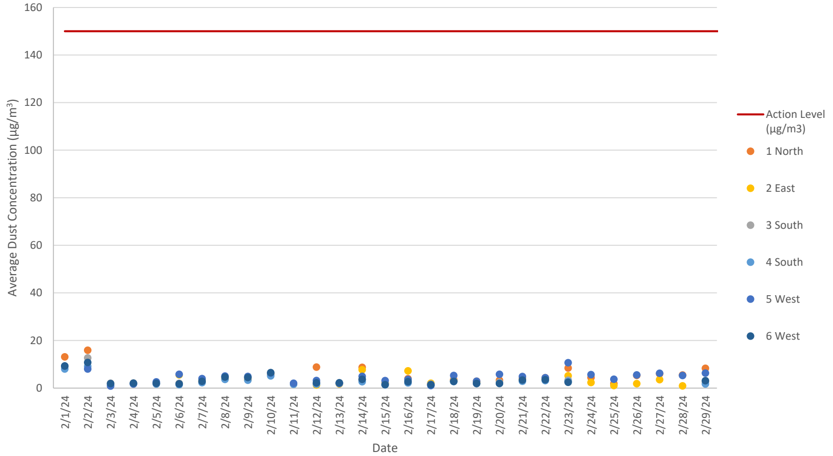
Figure 3 Dust Concentration 24-hour Averages February 1 - February 29, 2024 776 Summer Street Boston, Massachusetts
