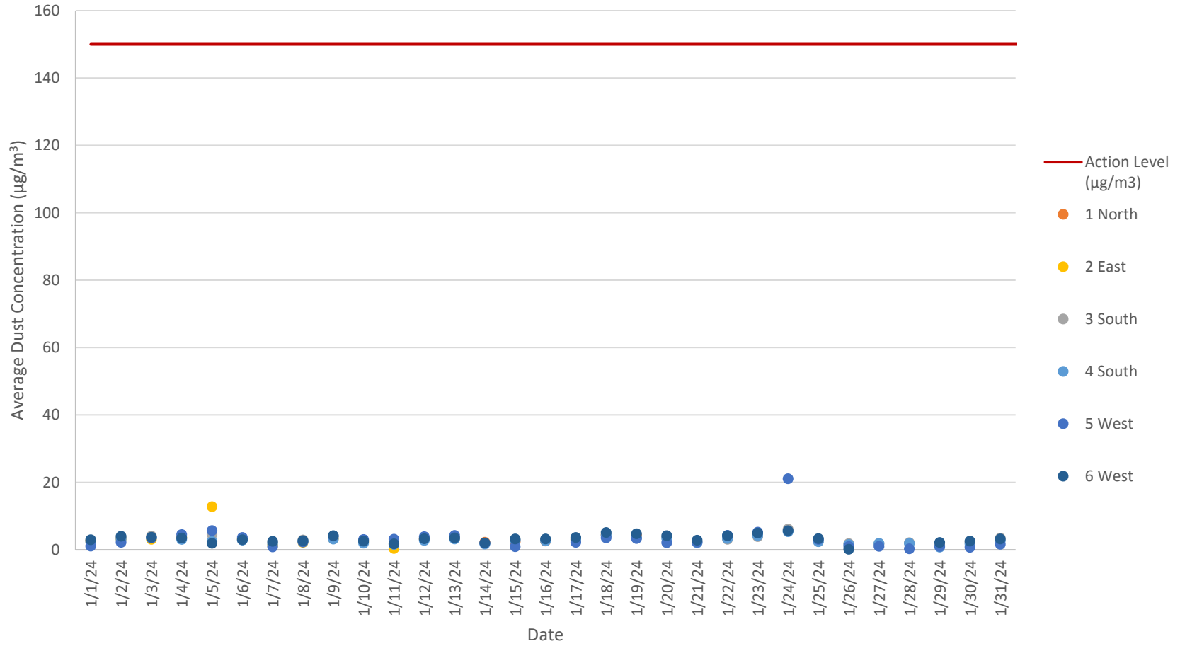
Figure 3 Dust Concentration 24-hour Averages January 1 - January 31, 2024 776 Summer Street Boston, Massachusetts
